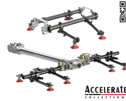
End Effector SpiderGrip™ geometrico
